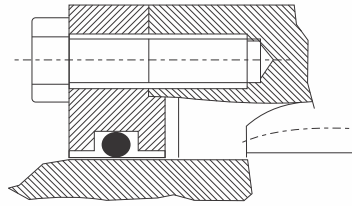
DETAIL 'X' THIS COVER PLATE CONSTRUCTION FOR SIZES UFG - 111 ONWARDS
